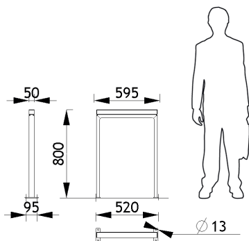
Link Bicycle guard Ref: 11 0560 - 7 kg
