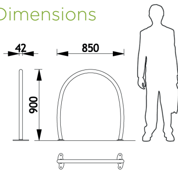
Large Arch Ref: 43 015x - 8 kg
