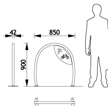
Large Arch with parking pattern plate Ref: 43 015x - 11 kg
