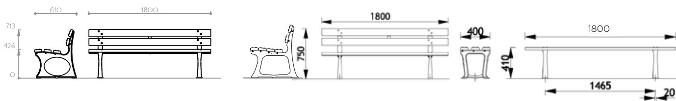
Confort 1 RRP seat Ref. 10 0002 PM1x OP00 - 66 kg
