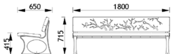
Confort 1 Nature seat 3 place seat - Ref. 13 1013 - 100 kg
