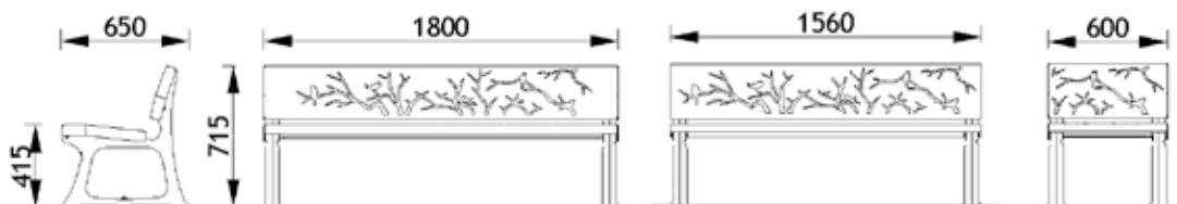
Confort 2 Nature seat 3 place seat - Ref. 13 1003 - 100 kg 2 place seat - Ref. 13 1002 - 85 kg Chair - Ref. 13 1001 - 36 kg
