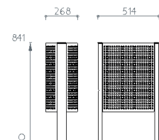
50-liters bin Ref: 20 0556N PLA Weight* with bag holder: 23 kg 50-liters bin Ref: 20 0555N PLA Weight* with liner: 27 kg
