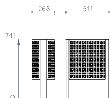
42-liters bin Ref: 20 0550N PLA Weight* with bag holder: 20 kg 38-liters bin Ref: 20 0551N PLA Weight* with liner: 24 kg
