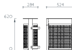
42-liters bin Ref: 20 0552N MUR Weight* with bag holder: 26 kg 38-liters bin Ref: 20 0553N MUR Weight* with liner: 30 kg
