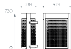
50-liters bin Ref: 20 0556N MUR Weight* with bag holder: 30 kg 46-liters bin Ref: 20 0557N MUR Weight* with liner: 4 kg
